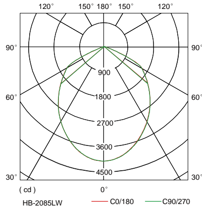
Bell-shaped lampshade – big (Ø420mm*255mm 60°) Weight: 0.7kg/ 1.54lb
