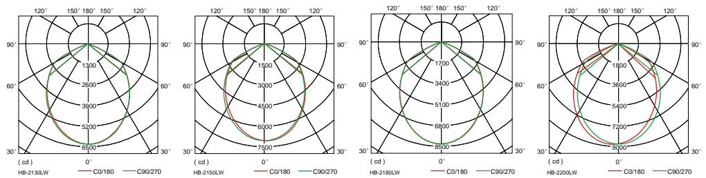
Bell-shaped lampshade – big (Ø420mm*255mm 60°) Weight: 0.7kg/ 1.54lb
